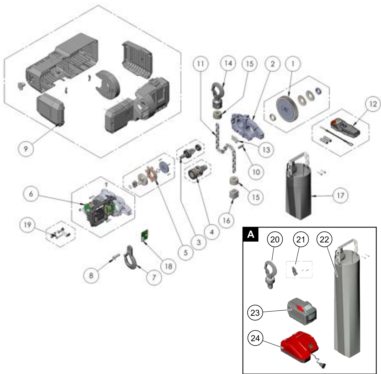
Figure 16. Hoist Parts
