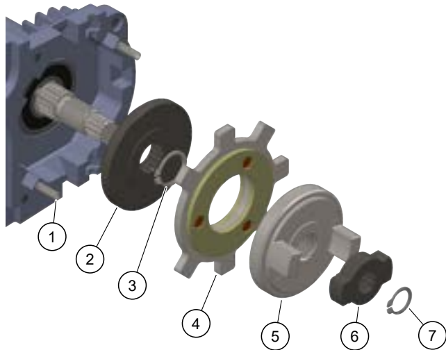
Figure 13. Brake Assembly
